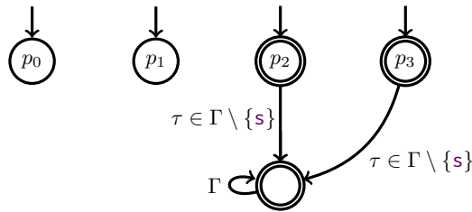
FIGURE 8.5 – Un \mathcal{P} -automate \mathcal{A} tel que \text{Conf}(\mathcal{A}) = \text{Err} .
